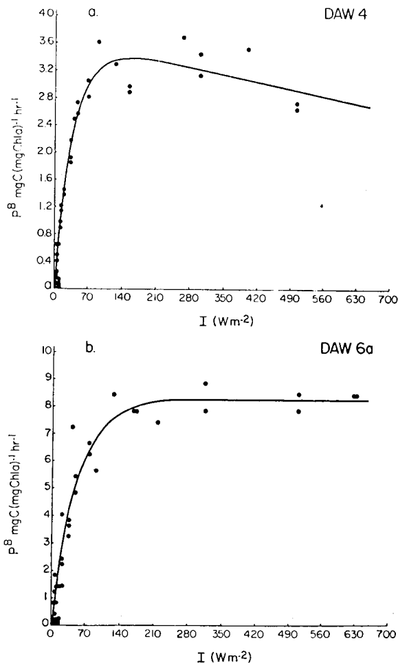
Fig. 4 Representative light-saturation experiments from the Nova Scotia Shelf. See Table 1.
