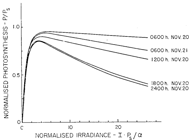
Fig. 8 Data of Fig. 6 replotted in scaled form.
