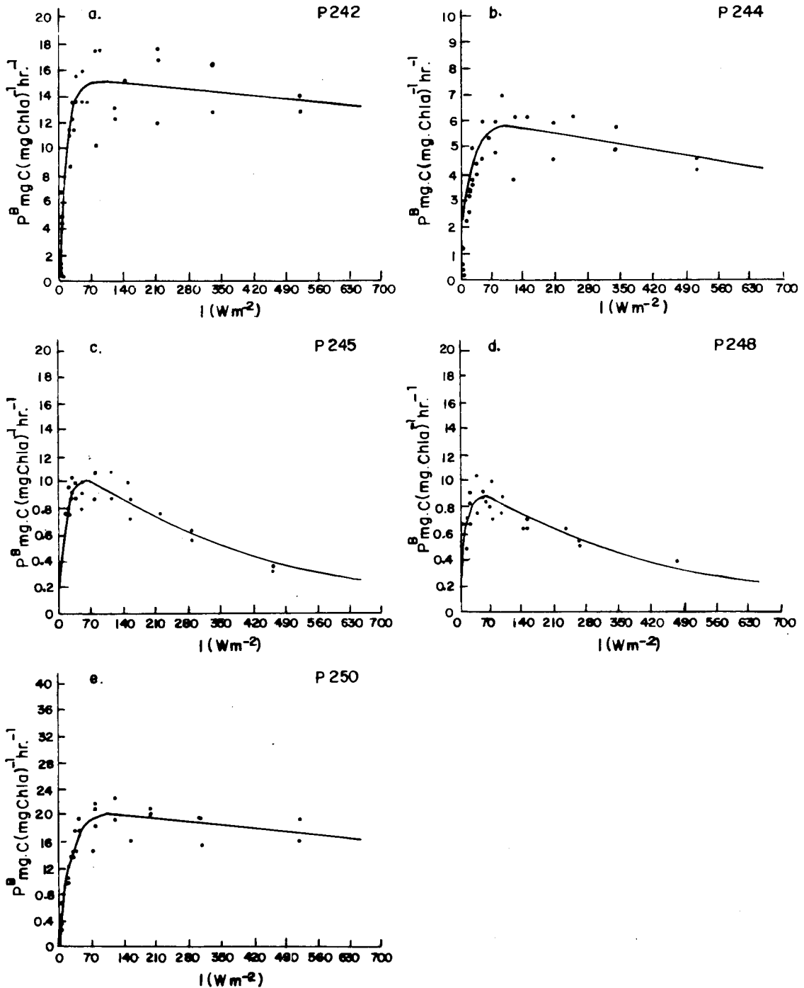
Fig. 6 Diurnal series of light-saturation experiments made off Peru. See Table 1.
