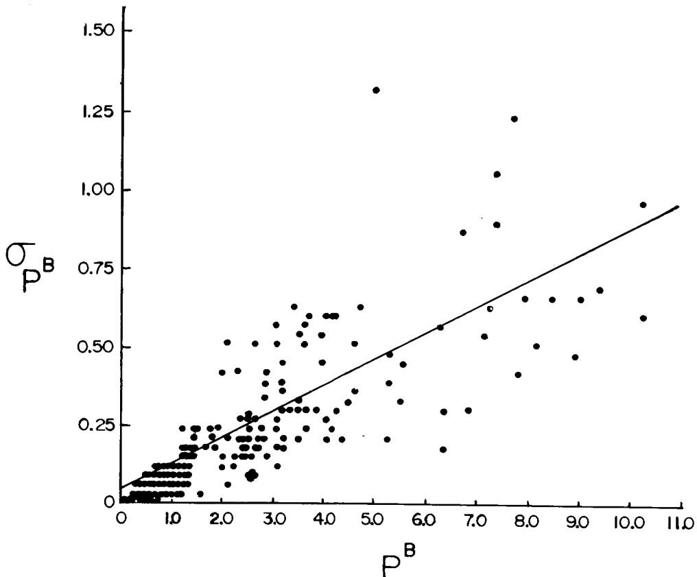
Fig. 2 Relationship between standard deviation and mean of specific production rate for natural assemblages of coastal marine phytoplankton. Data from Therriault et al., 1978.
