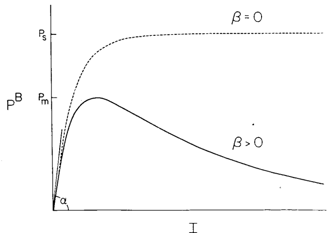
Fig.1 General form of the function described by equation (1).
