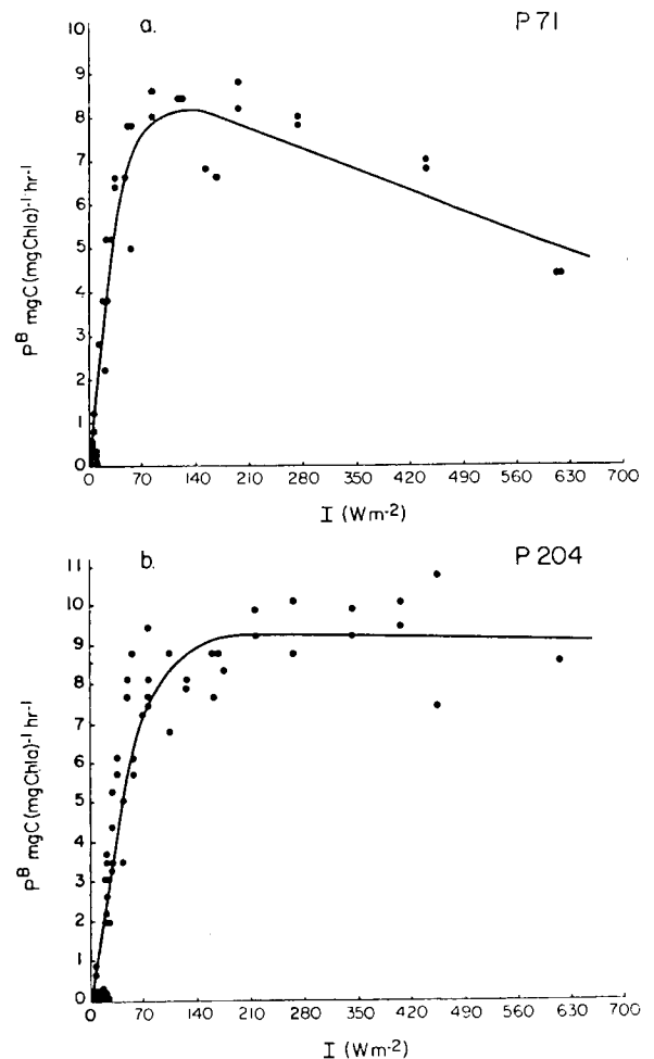
Fig. 3 Representative light-saturation experiments from Peru. See Table 1.
