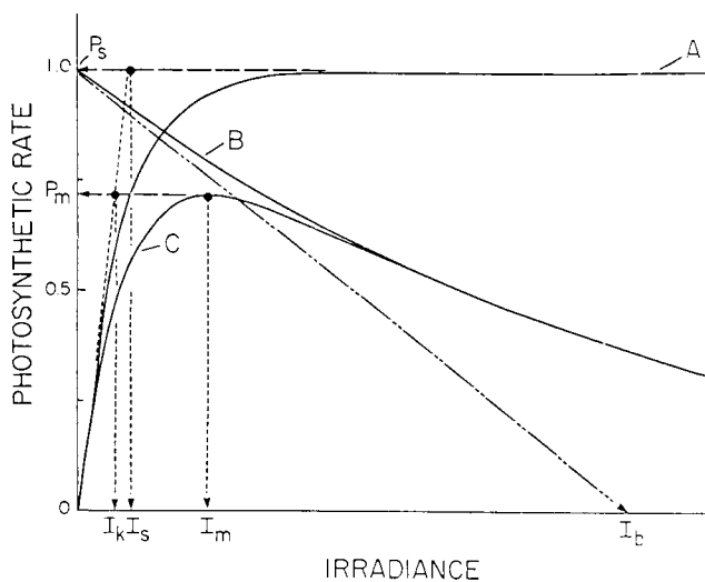
Fig. 7 Showing the geometric relationships of the photosynthetic parameters and derived parameters.
